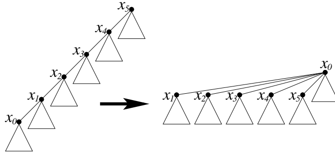
Figure 12.1: Reversal of the path x_0, x_1, x_2, x_3, x_4, x_5 .
