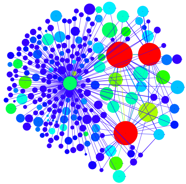
Fig. 9. An egocentric visualization of the vertex representing WikiLeaks’ public-key in the imperfect user network. The size of a vertex corresponds to its degree in the entire imperfect user network. The color denotes the volume of Bitcoins – warmer colors have larger volumes flowing through them. The large red vertices represent a Bitcoin mining pool, a centralized Bitcoin wallet service and an unknown entity.
