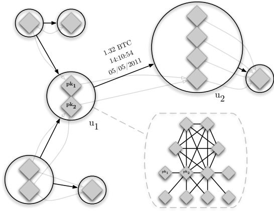
Fig. 6. An example sub-network from the user network. Each circular vertex represents a user and each directed edge between circular vertices represents a flow of Bitcoins from one user to another. The maximal connected component from the ancillary network that corresponds to the vertex u_1 is shown within the dashed grey box.
