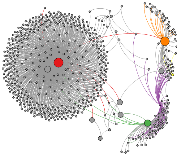
Fig. 11. An egocentric visualization of the thief in the imperfect user network. For this visualization, vertices are identified through their colors in the text, edges are colored according to the color of their sources and the size of each vertex is proportional to its edge-betweenness within the egocentric network.
