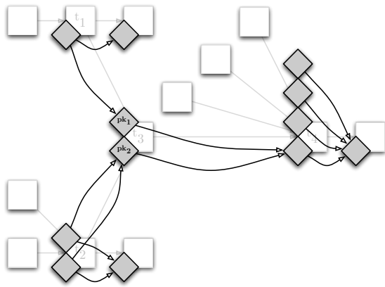
Fig. 5. An example sub-network from the imperfect network. Each diamond vertex represents a public-key and each directed edge between diamond vertices represents a flow of Bitcoin from one public-key to another.
