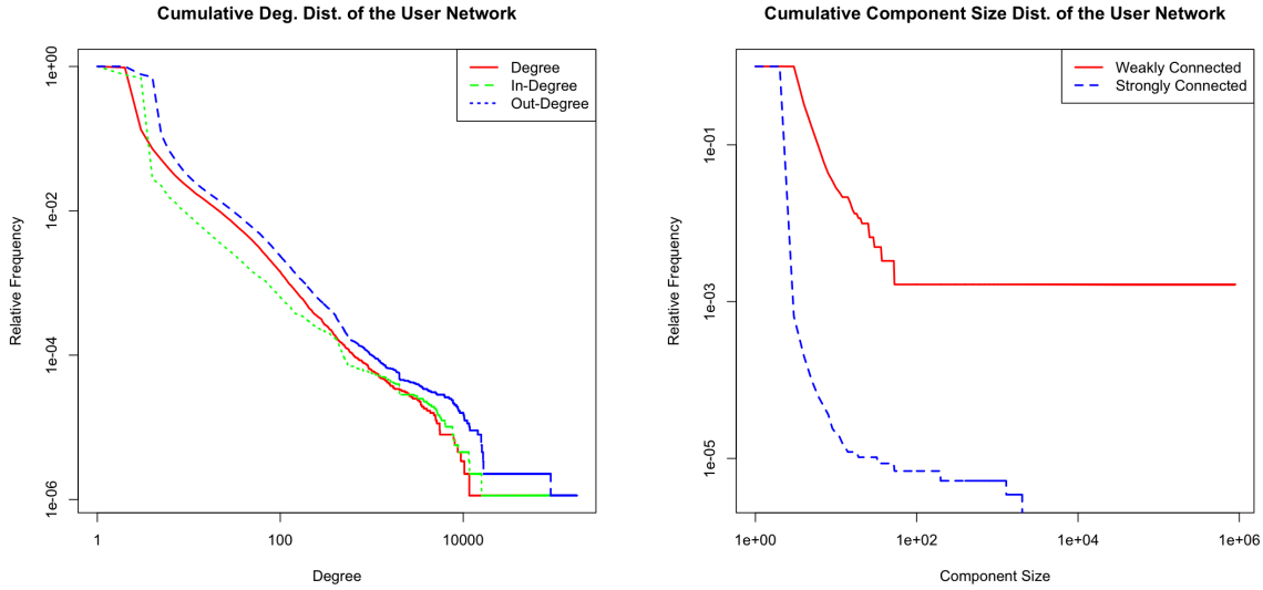
(a) A log-log plot of the cumulative degree distributions. (b) A log-log plot of the cumulative component size distribution.
