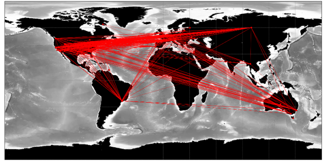
(b) A map of a sample of the geolocated IP addresses in Fig. 7(a) connected by edges where the corresponding users are connected by a path of length at most three in the user network that does not include the vertex representing the Bitcoin Faucet.
