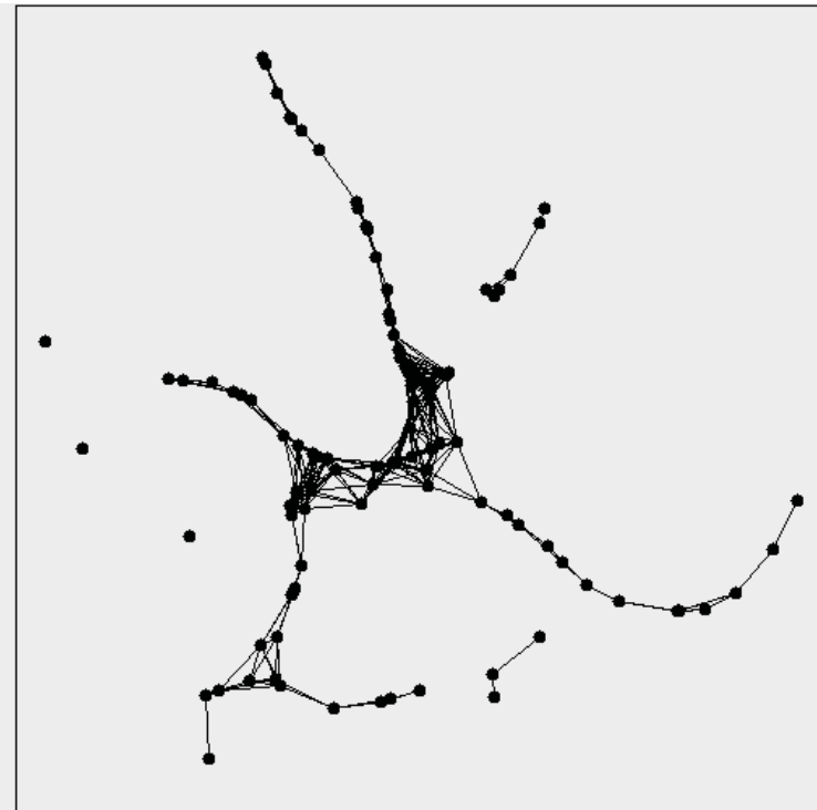
Network graph
