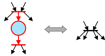
Fusion of Series Transitions (FST)
