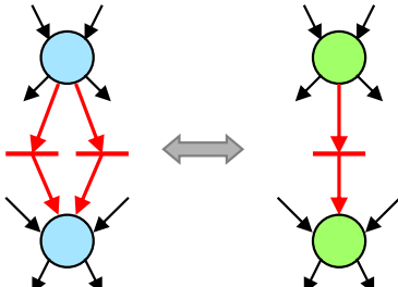
Fusion of Parallel Transitions (FPT)
