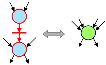
Fusion of Series Places (FSP)
