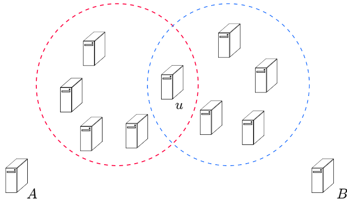
Figure 4: An unfortunate case with a simple byzantine node can lead to disagreement!
