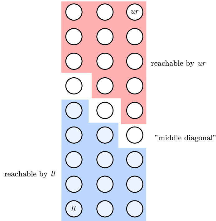
Figure 5: A grid with w = 2 and h = 8 .
