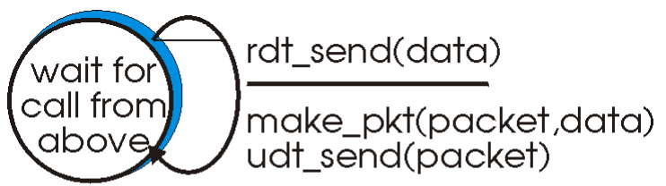
(a) rdt 1.0: sending side
