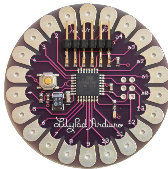
Figure 1: LilyPad Arduino
