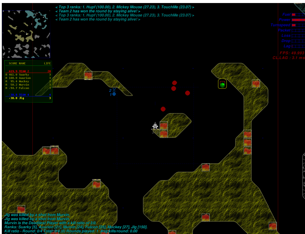
Figure 2.1: x-pilot-ng-sdl screenshot.
