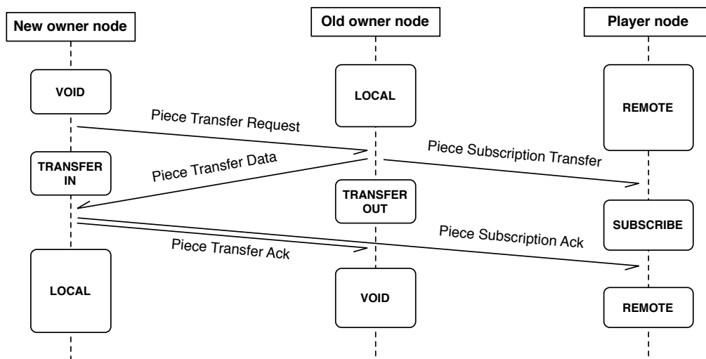
Figure 3.8: Combined piece transfer and subscription transfer process involving three distinct nodes. Messages are sent asynchronously.
