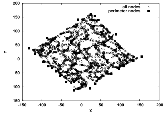
Figure 5: The virtual coordinates of a network with 3200 nodes where no node knows its coordinates or whether it is on the perimeter.
