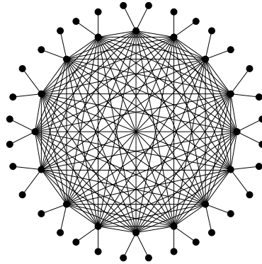
Figure 5.2: Distributed greedy algorithm with rounded spans: Bad example
