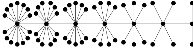
Figure 5.1: Distributed greedy algorithm: Bad example
