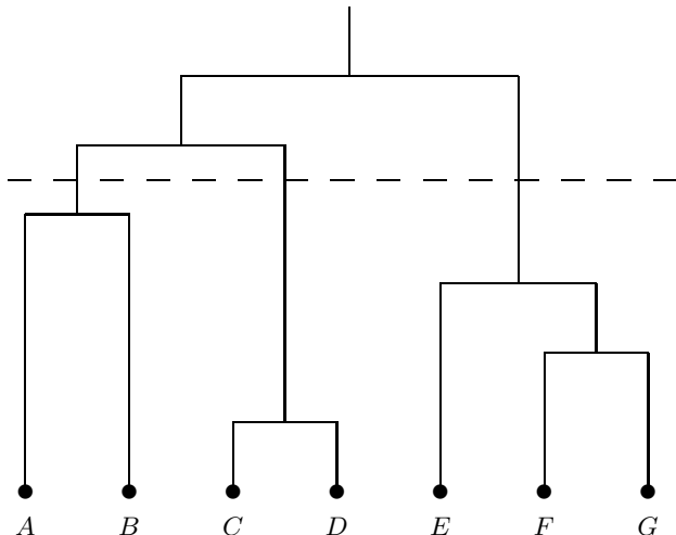
Figure 1: A dendrogram representation of a hierarchical clustering of points A through G . For any k , we can read off the k -clustering associated with the hierarchical clustering by visualizing a horizontal line that cuts k vertical lines of the dendrogram, thereby partitioning the leaves into k sets. For example, the dashed line shown above induces the 3-clustering \{\{A, B\}, \{C, D\}, \{E, F, G\}\} .
