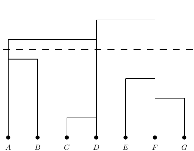
Figure 2: The above dendrogram variant encodes a hierarchical ordering in which F has rank 0 and parent F , D has rank 1 and parent F , A has rank 2 and parent D , B has rank 3 and parent A , E has rank 4 and parent F , G has rank 5 and parent F , and C has rank 6 and parent D . The dashed line induces the idempotent 3-assignment in which A and B are mapped to A , C and D are mapped to D , and the three remaining points are mapped to F .
