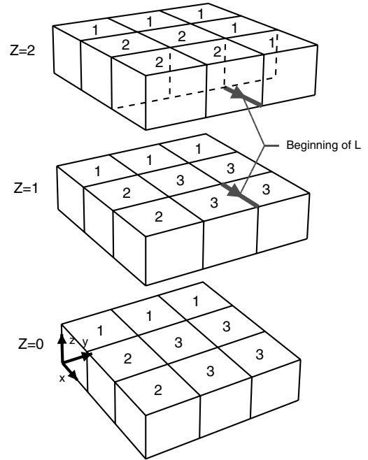
Figure 2: The 27 cubelets around the beginning of line L .
