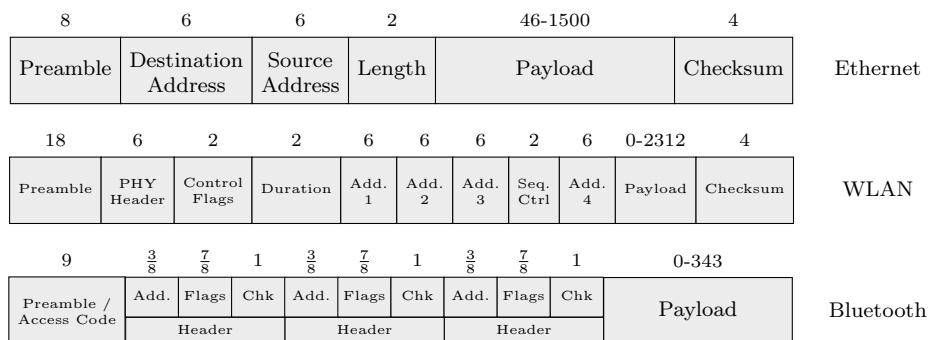
Figure 10.31: The complete physical representations of typical Ethernet, Wireless LAN and Bluetooth packets. The number above each field corresponds to its length in bytes.
