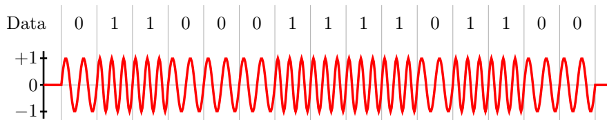
Figure 10.46: Frequency modulation.
