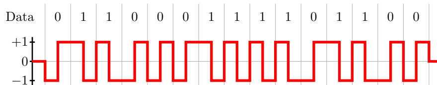
Figure 10.41: Manchester coding.
