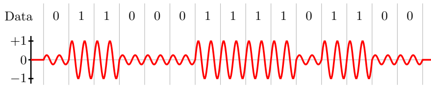
Figure 10.44: Amplitude modulation.
