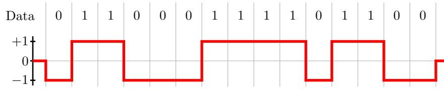
Figure 10.39: Simple line coding.
