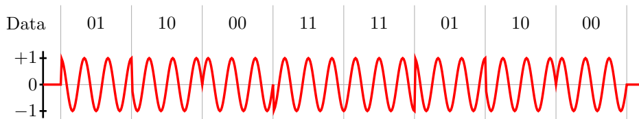
Figure 10.48: Phase modulation with 2-bit symbols.
