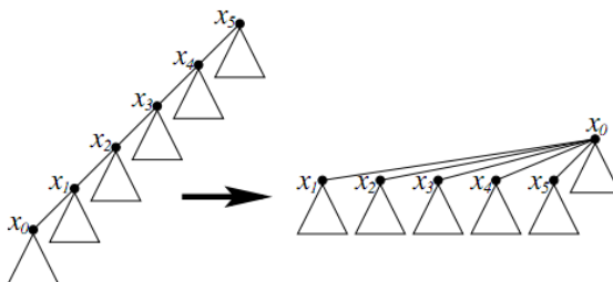
Figure 3.11: Reversal of the path x_0, x_1, x_2, x_3, x_4, x_5 .
