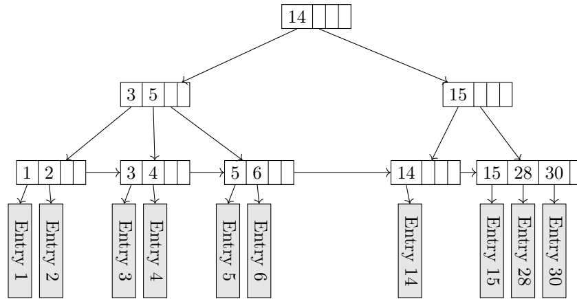
Figure 7.26: Example B+ tree of order b = 4 .
