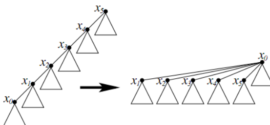
Figure 7.11: Reversal of the path x_0, x_1, x_2, x_3, x_4, x_5 .
