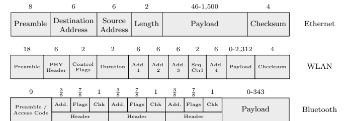
Figure 5.3: The complete physical representations of typical Ethernet, Wireless LAN and Bluetooth packets. The number above each field corresponds to its length in bytes.
