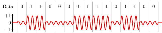
Figure 5.25: Amplitude modulation.
