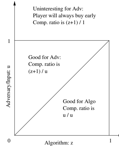
Figure 1: Choosing more than two values
