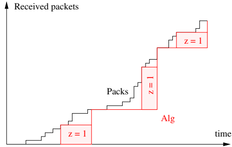
Figure 3: The z = 1 algorithm
