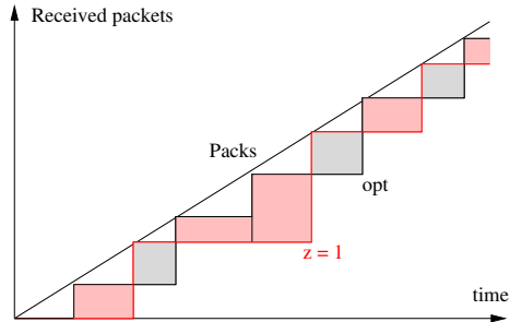
Figure 4: A_{z=1} vs. the optimal algorithm
