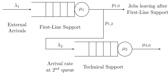
Figure 6.28: A queueing network modeling a two-tier support hotline. Jobs arrive from the outside with rate \lambda_1 and enter the queue for first-line support. After the first-line support served the job, with rate \mu_1 , a p_{1,0} = (1 - p_{1,2}) fraction of the jobs are satisfied and leave the system. The remaining p_{1,2} fraction of jobs need in-depth technical assistance, which is provided by a technician in the technical support queue. Technical support takes time exponentially distributed with parameter \mu_2 , and afterwards the job leaves the system.
