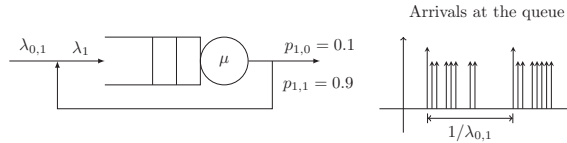
Figure 6.30: A queueing network exhibiting bursty behaviour. External jobs arrive with rate \lambda_{0,1} , and jobs leaving the queueing system immediately re-enter with probability p_{1,1} = 0.9 . Thus, in expectation, each job enters the queue 10 times before leaving the system. The external arrivals at the queue, indicated as long arrows in the right graph, are a Poisson process. However, the total arrivals at the queue are not Poisson—after serving an external arrival the job is likely to loop back to the queue a few times.
