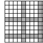
Figure 15.31: An example how to choose a quorum in the M -Grid with f = 3 , i.e., 2 rows and 2 columns. The load is in \Theta(\sqrt{f}/n) when the access strategy is chosen to be uniform. Two quorums overlap with each row intersecting each other's column, i.e., 2\sqrt{f+1}^2 = 2f+2 nodes.
