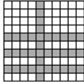
Figure 15.29: An example how to choose a quorum in the f -masking Grid with f = 2 , i.e., 2+1 = 3 rows. The load is in \Theta(f/\sqrt{n}) when the access strategy is chosen to be uniform. Two quorums overlap by their columns intersecting each other's rows, i.e., they overlap in at least 2f+2 nodes.
