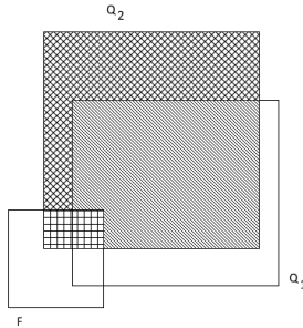
Figure 15.34: Intersection properties of an opaque quorum system. Equation (15.33.1) ensures that the set of non-byzantine nodes in the intersection of Q_1, Q_2 is larger than the set of out of date nodes, even if the byzantine nodes “team up” with those nodes. Thus, the correct up to date value can always be recognized by a majority voting.
