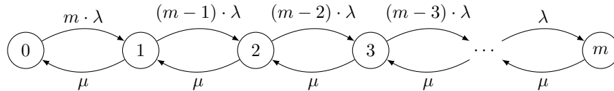
Figure 8.27: Birth-Death process modeling an M/M/1/m/m queueing system.
