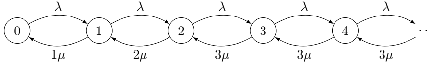
Figure 8.25: Birth-Death process modeling an M/M/3 queueing system. If there are less than 3 jobs, then the number of active servers is the number of jobs in the system. When 3 or more jobs are in the system all servers are active.
