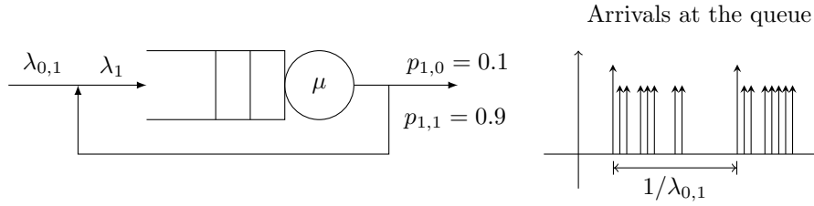
Figure 8.30: A queueing network exhibiting bursty behaviour. External jobs arrive with rate \lambda_{0,1} , and jobs leaving the queueing system immediately re-enter with probability p_{1,1} = 0.9 . Thus, in expectation, each job enters the queue 10 times before leaving the system. The external arrivals at the queue, indicated as long arrows in the right graph, are a Poisson process. However, the total arrivals at the queue are not Poisson—after serving an external arrival the job is likely to loop back to the queue a few times.
