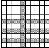
Figure 21.29: An example how to choose a quorum in the f -masking Grid with f=2 , i.e., 2+1=3 rows. The load is in \Theta(f/\sqrt{n}) when the access strategy is chosen to be uniform. Two quorums overlap by their columns intersecting each other's rows, i.e., they overlap in at least 2f+2 nodes.
