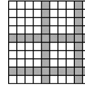
Figure 21.31: An example how to choose a quorum in the M -Grid with f=3 , i.e., 2 rows and 2 columns. The load is in \Theta(\sqrt{f}/n) when the access strategy is chosen to be uniform. Two quorums overlap with each row intersecting each other's column, i.e., 2\sqrt{f+1}^2 = 2f+2 nodes.
