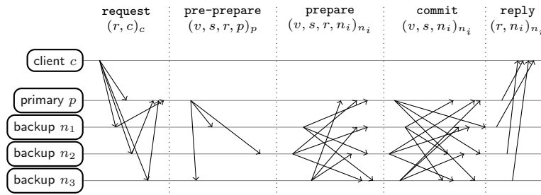
Figure 25.9: The agreement protocol used in PBFT for processing a client request issued by client c , exemplified for a system with n = 4 nodes. The primary in view v is p = n_0 = v \bmod n .
