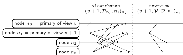
Figure 25.21: The view change protocol used in PBFT. Node n_0 is the primary of current view v , node n_1 the primary of view v + 1 . Once backups consider n_0 to be faulty, they start the view change protocol (cf. Algorithms 25.23, 25.24, 25.25). The X signifies that n_0 is faulty.
