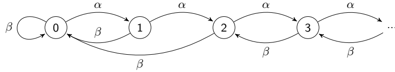
Figure 25.4: Each state of the Markov chain represents how many blocks the selfish miner is ahead, i.e., d_s - d_p . In each state, the selfish miner finds a block with probability \alpha , and the honest miners find a block with probability \beta = 1 - \alpha . The interesting cases are the “irregular” \beta arrow from state 2 to state 0, and the \beta arrow from state 1 to state 0 as it will include three subcases.
