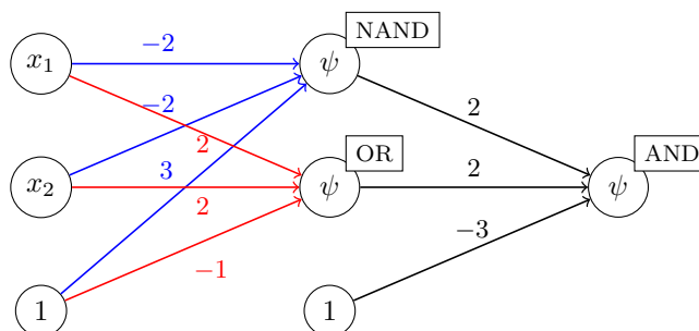
Figure 3: Hierarchical Logistic Regression for “XOR”
