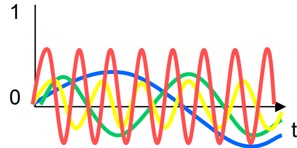
superpose harmonics
