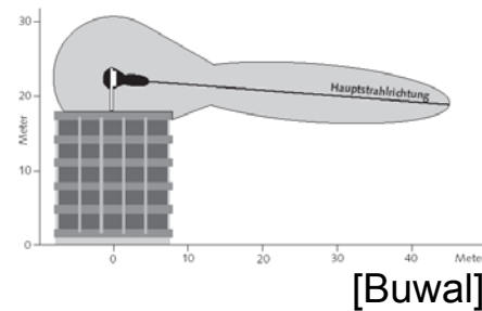
directed antenna
